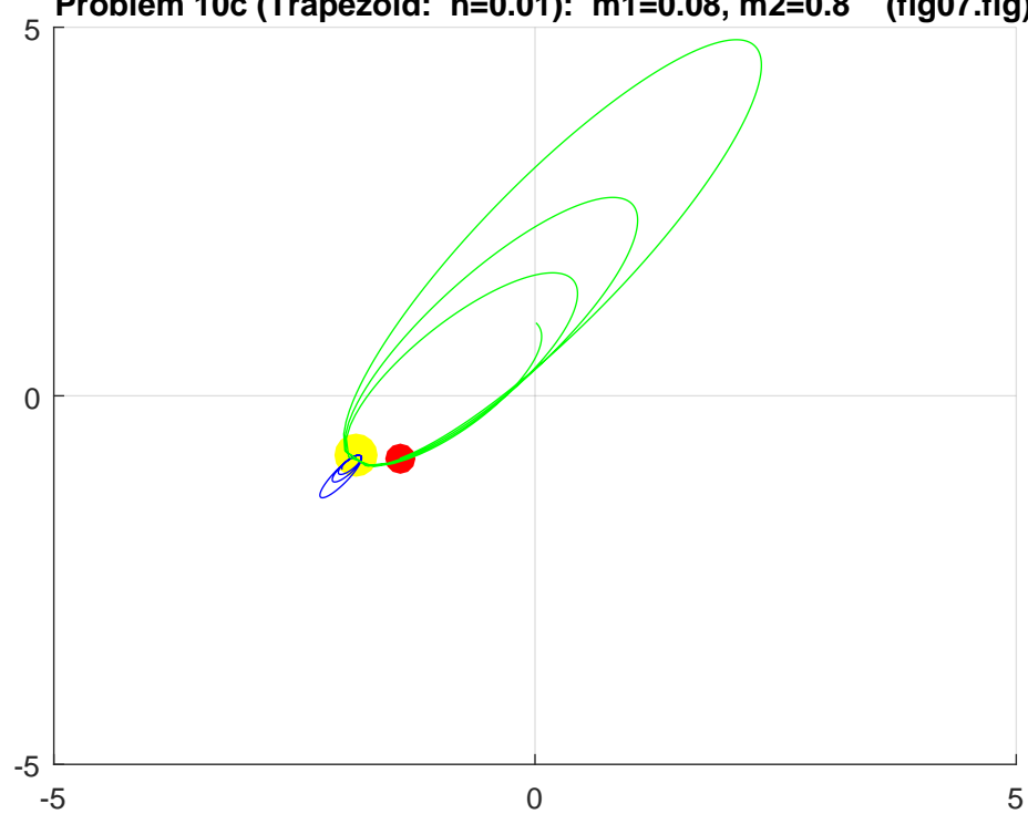
Celestial Mechanics: Two (2) Body Problem Problem 10c (Trapezoid: h=0.01 ): m_1=0.08 , m_2=0.8 (fig07.fig)
